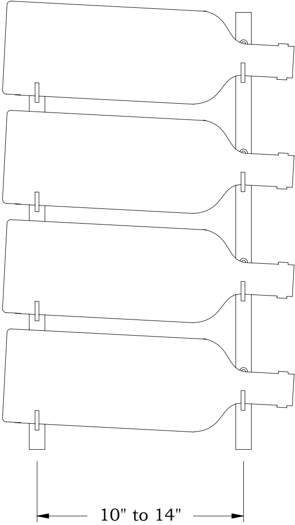
(Standard Mounting) Front View
